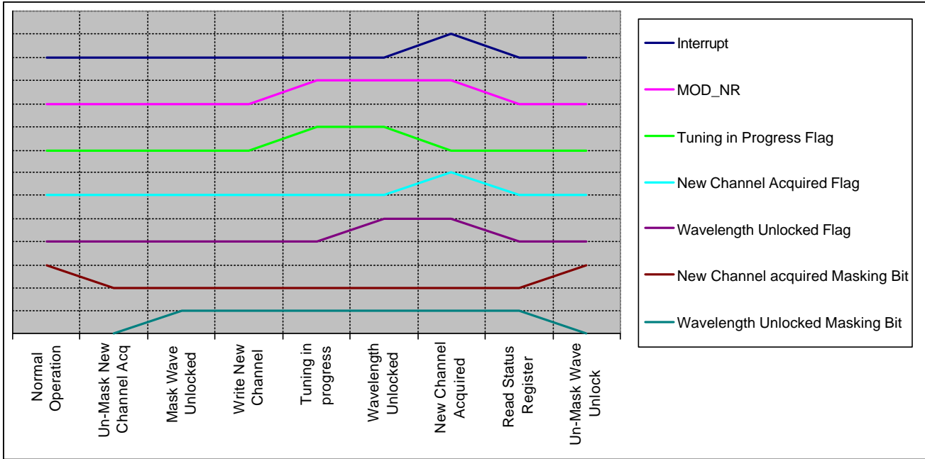
Timing diagram for channel-to-channel switching.
